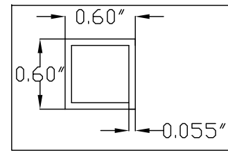
425 RESIDENTIAL PICKET
