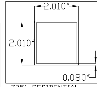
7751 RESIDENTIAL POST
