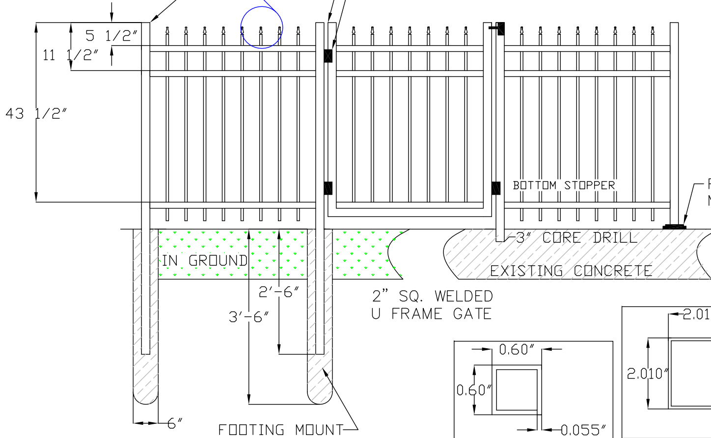
7751 RESIDENTIAL POST
