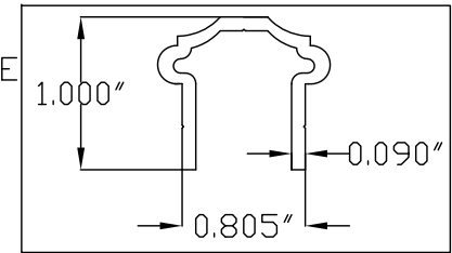
1119 RESIDENTIAL CHANNEL
