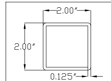
304 GATE POST
