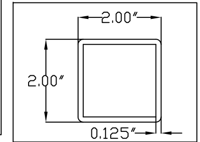
304 GATE POST
