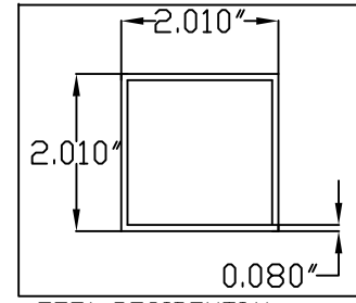
7751 RESIDENTIAL POST
