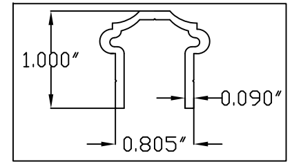
1119 RESIDENTIAL CHANNEL
